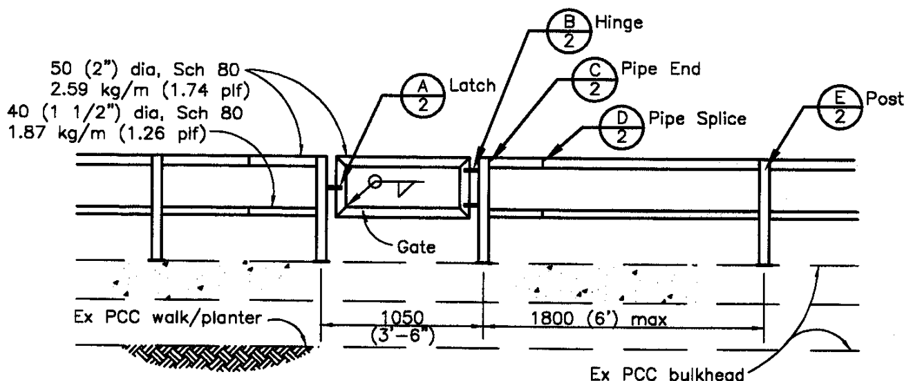
TYPICAL ELEVATION
